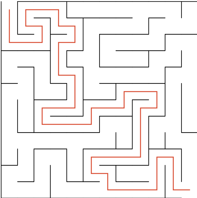
Maze 15
