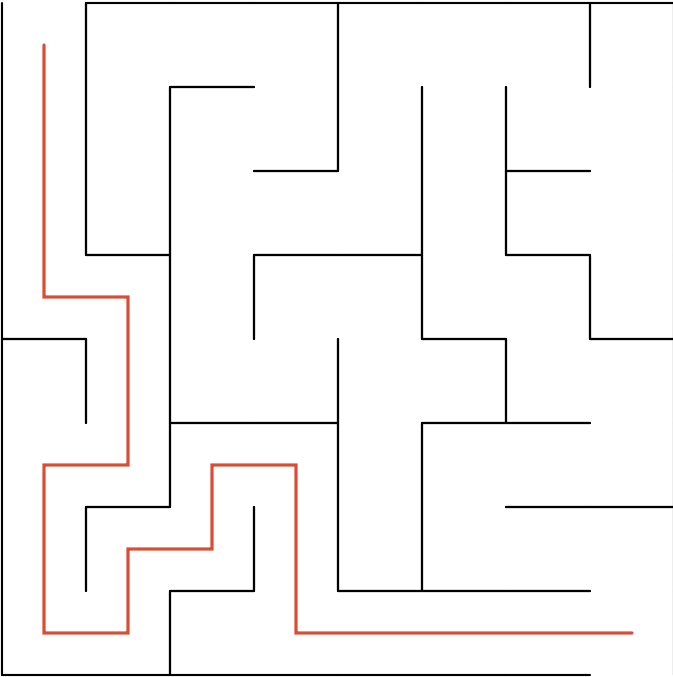
Maze 5
