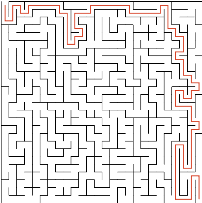
Maze 47
