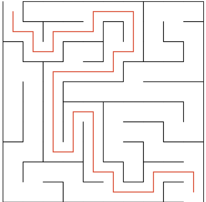
Maze 8
